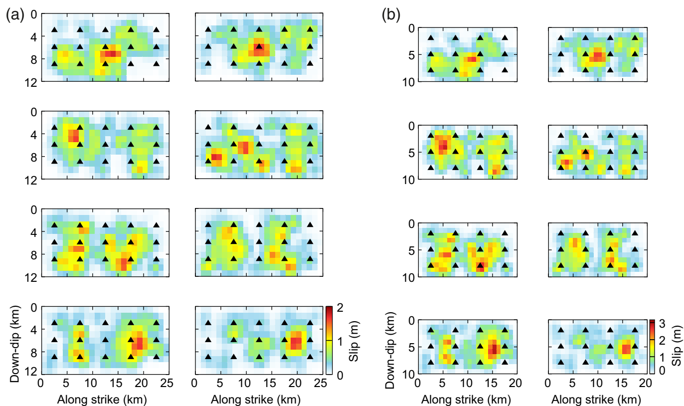
Figure 2. Eight slip distributions used in the scenario source modeling obtained by changing the distribution of sub-sources of the Hybrid Integral–Composite (HIC) model for fault sizes (a) 25 \times 12 km 2 and (b) 20 \times 10 km 2 . The largest sub-sources are placed deterministically to simulate various positions of asperities, whereas the others are distributed randomly along the fault. The black triangles mark nucleation points from which the rupture propagates at constant speeds. Note the different color scales in the two panels. The color version of this figure is available only in the electronic edition.
