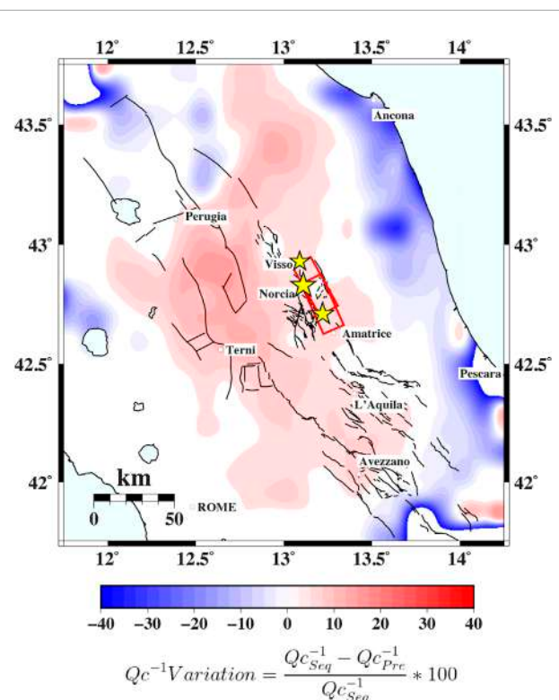
FIGURE 8 Percentage difference of Q_c^{-1} between the pre-sequence and sequence phases. Black lines are the faults from the ITHACA catalog. Red Line is the Monti Sibillini Thrust (MST).
