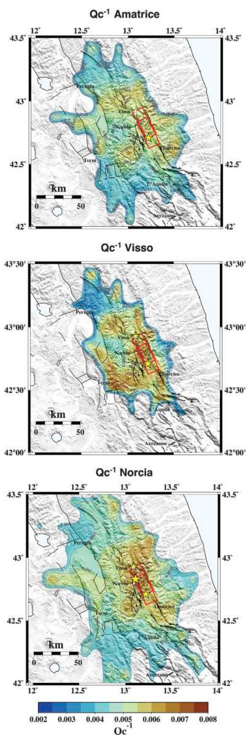
FIGURE 7 Spatial and temporal variation of Q_c^{-1} at f_c = 1.5 Hz for the sequences of Amatrice, Visso, and Norcia. Black lines are the faults from the ITHACA catalog. Red boxes are the fault plane for the Amatrice and Norcia earthquakes. The stars indicate the mainshocks of each 2016–2017 sequence.
