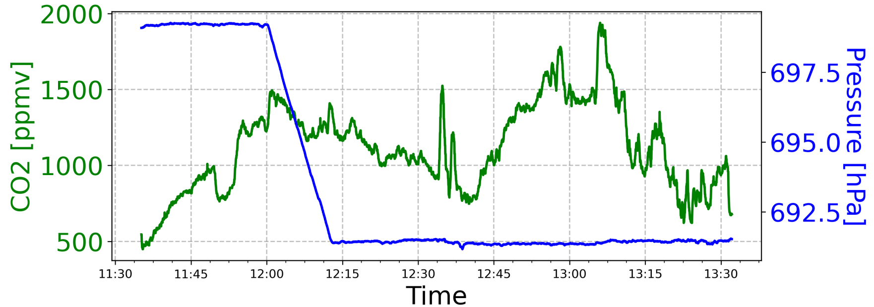
Volcanosonde Measurements | 1D - 05/06/2025 | Crater
