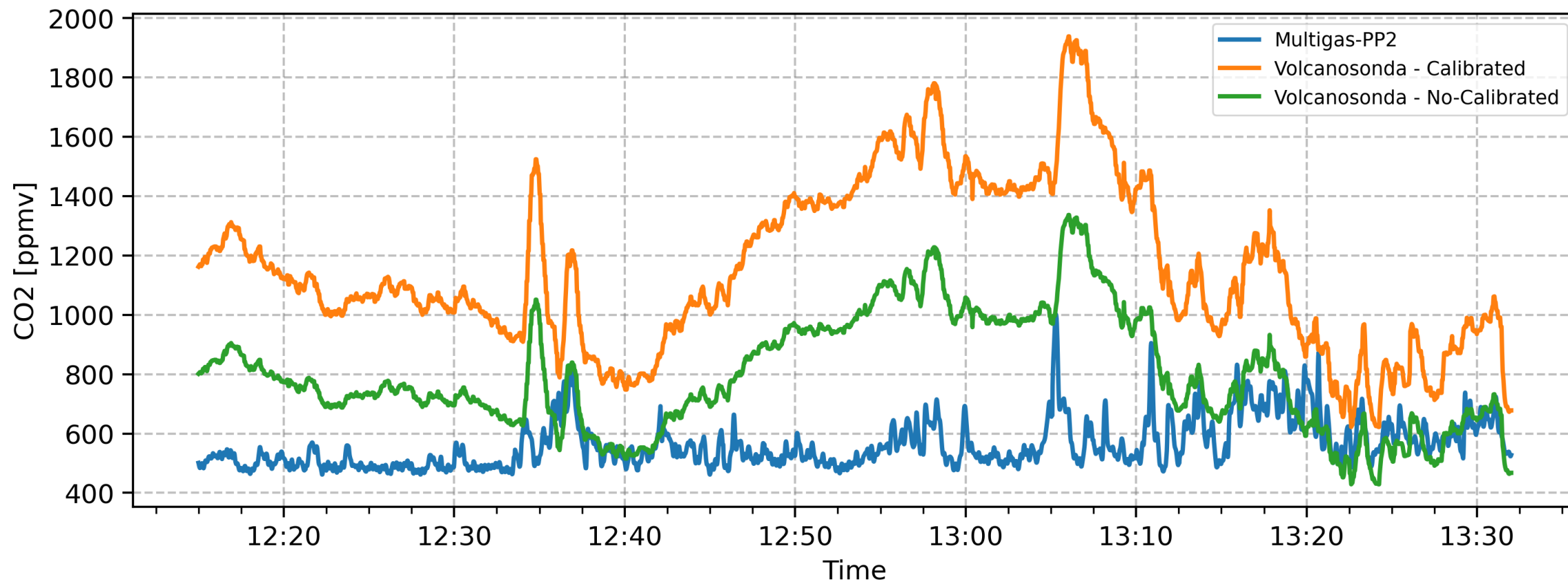
CO 2 Measurements Comparison | 05/06/2025 | Crater
