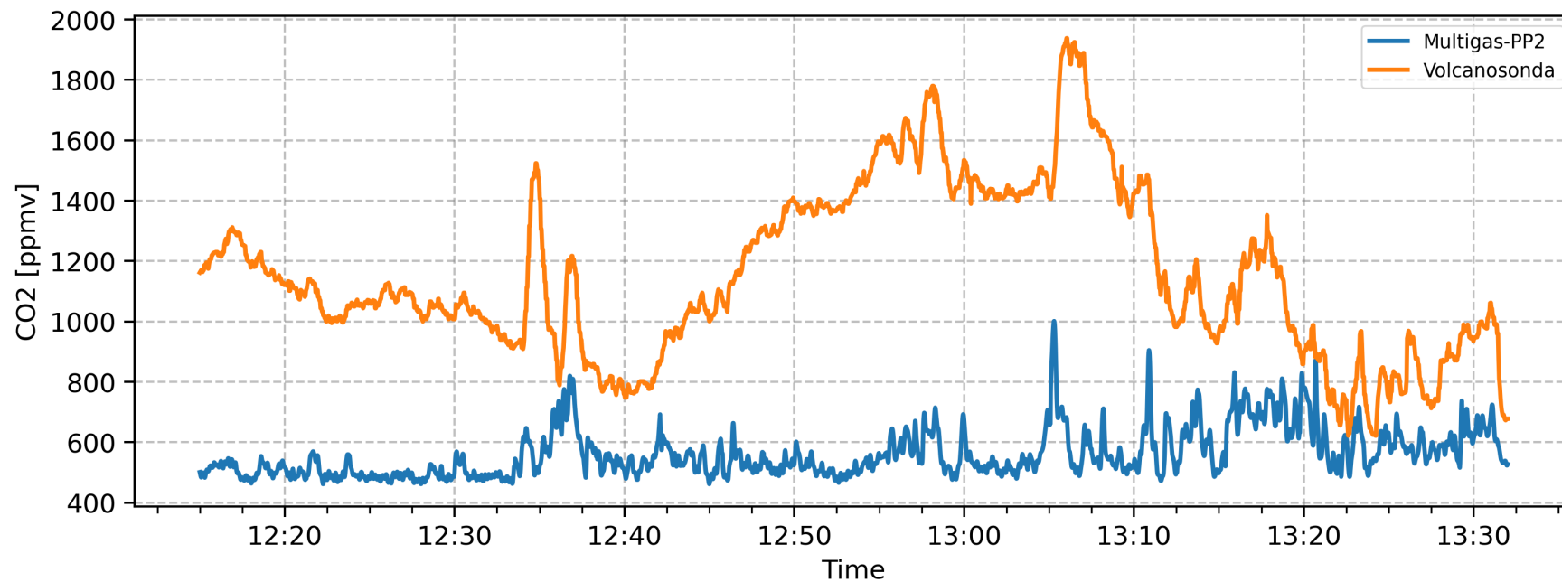
CO 2 Measurements Comparison | 05/06/2025 | Crater
