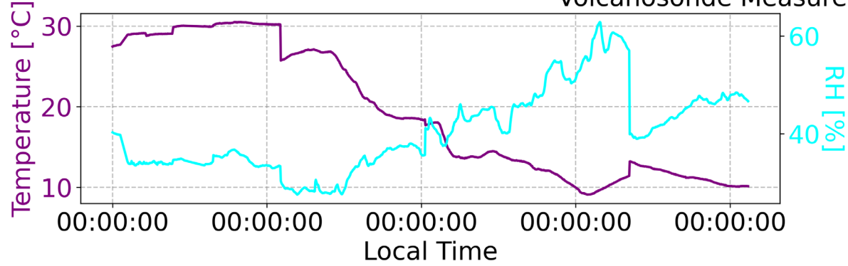
Volcanosonde Measurements | Drone - 06/06/2025
