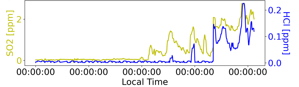
Volcanosonde Measurements | Drone - 06/06/2025
