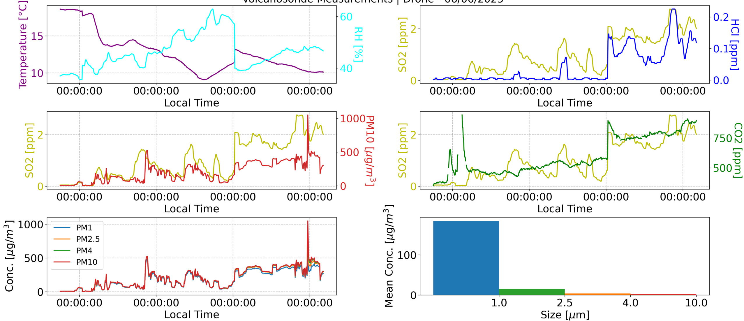
Volcanosonde Measurements | Drone - 06/06/2025
