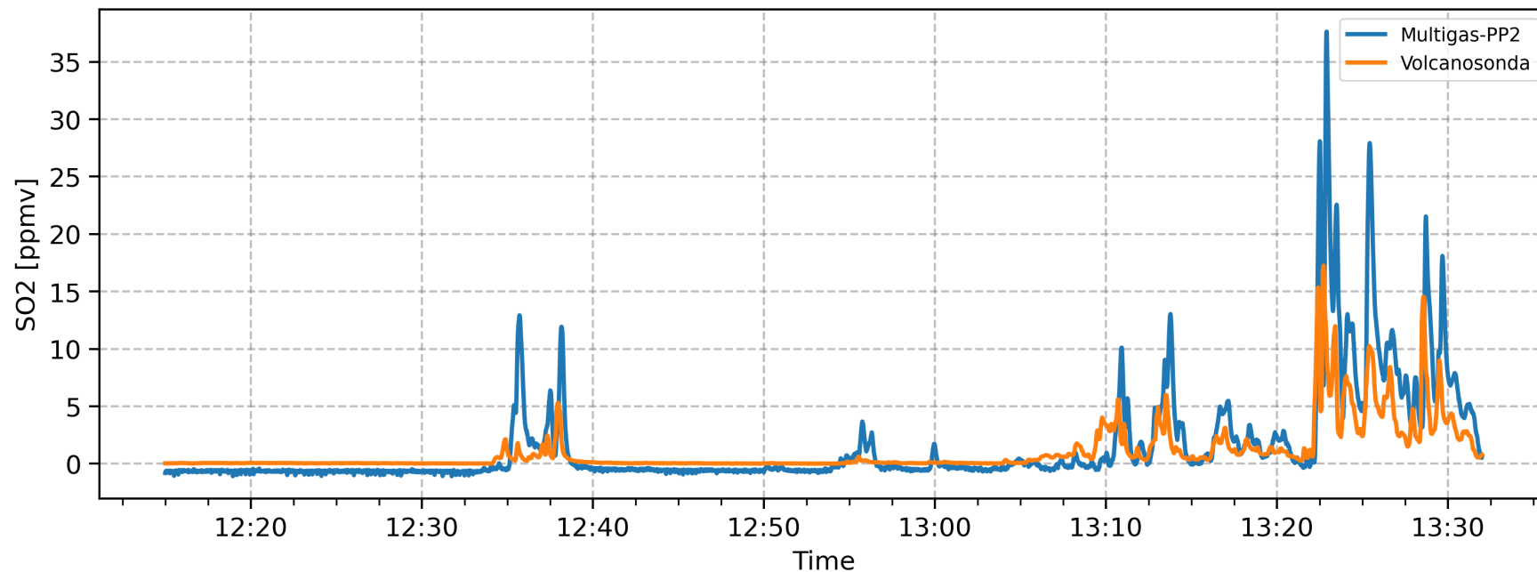
SO 2 Measurements Comparison | 05/06/2025 | Crater
