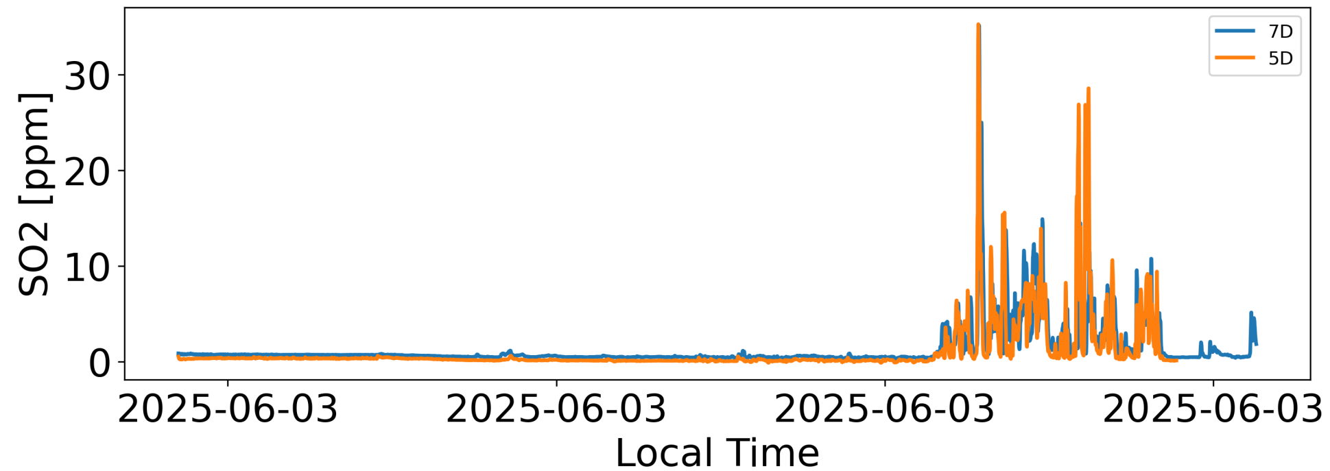
Volcanosonde Measurements | 5D and 7D - 03/06/2025
